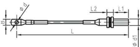
design B with socket
