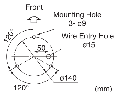
Mounting Dimension
