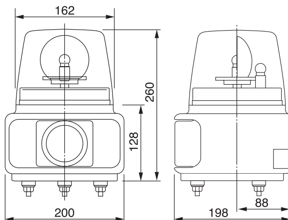
Mounting Dimension
