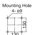
Mounting Dimension
