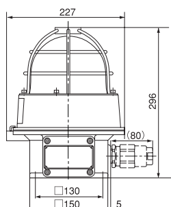
Mounting Dimension
