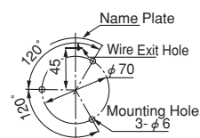
Mounting Dimensions
