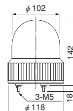
Mounting Dimensions
