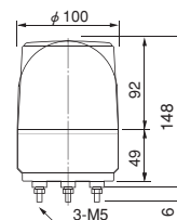
Mounting Dimensions
