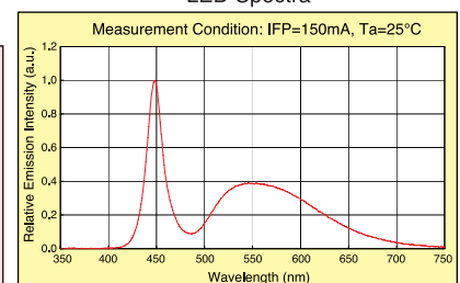
LED Spectra
