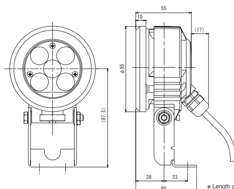
Mounting Dimension
