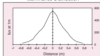
Illuminance Distribution
