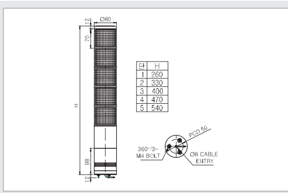
외형도 (External view drawing)
