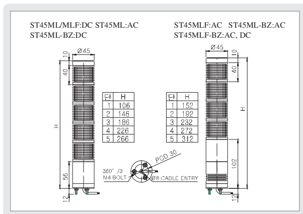
외형도 (External view drawing)
