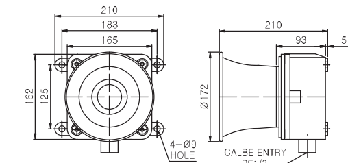
외형도 (External view drawing)
