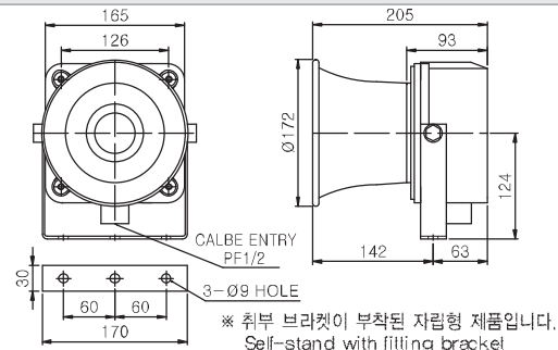
외형도 (External view drawing)
