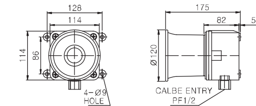
외형도 (External view drawing)
