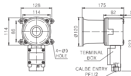
외형도 (External view drawing)
