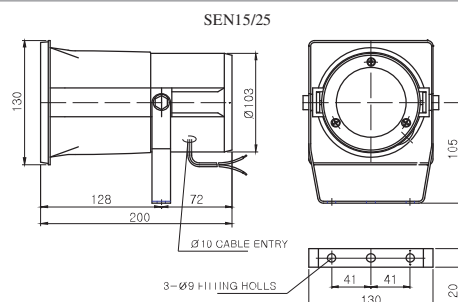
외형도 (External view drawing)
