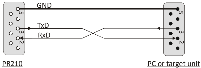
RS232 communication with PC or serial target unit
